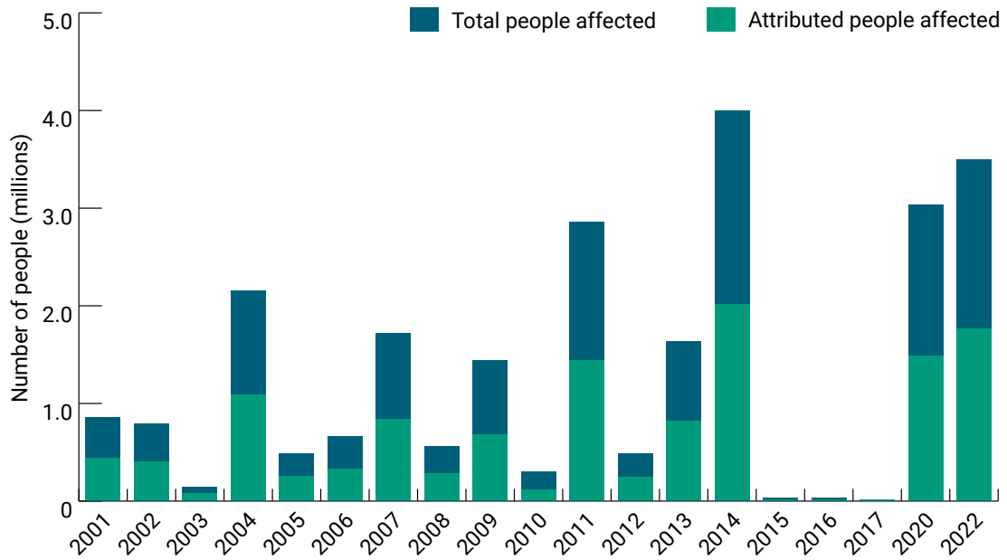
FIGURE 4: NUMBER OF DEATHS AND PEOPLE AFFECTED FROM DROUGHTS AND FLOODS IN SOMALIA
