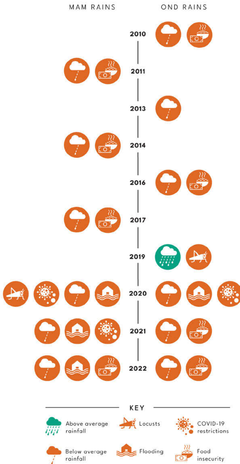
FIGURE 5: SHOCK TIMELINE IN SOMALIA, 2019–2022
