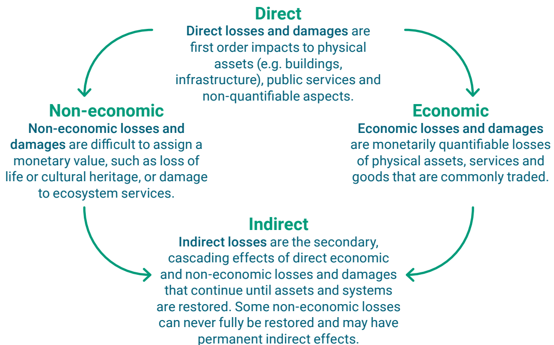
FIGURE 1: DIMENSIONS OF LOSS AND DAMAGE FROM EXTREME EVENTS AND SLOW-ONSET PROCESSES
