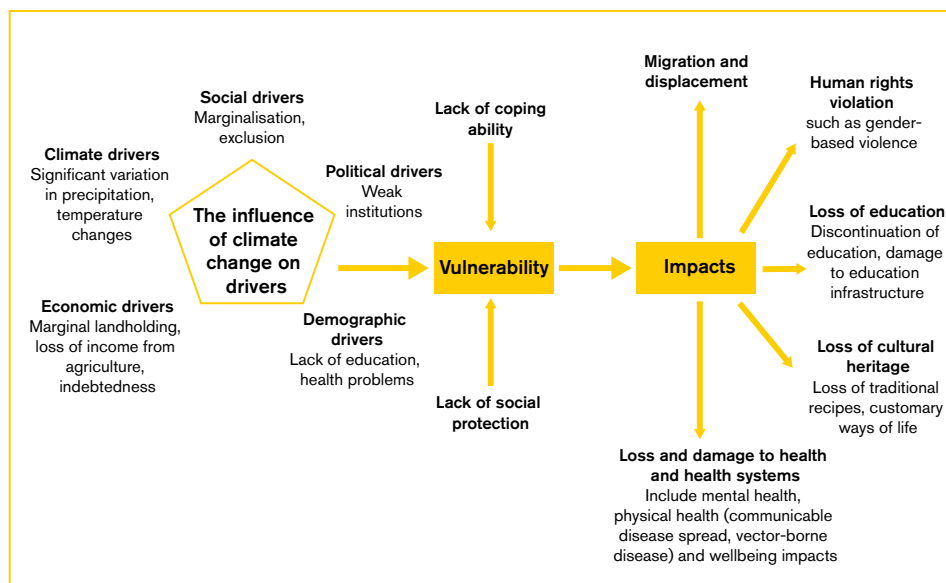
FIGURE 2: VULNERABILITY AND CLIMATE EVENTS LEADS TO IMPACTS
