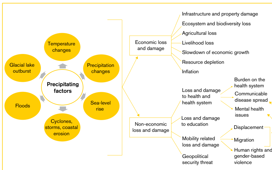
FIGURE 3: EXTREME AND SLOW-ONSET EVENTS TRIGGER LOSSES AND DAMAGES
