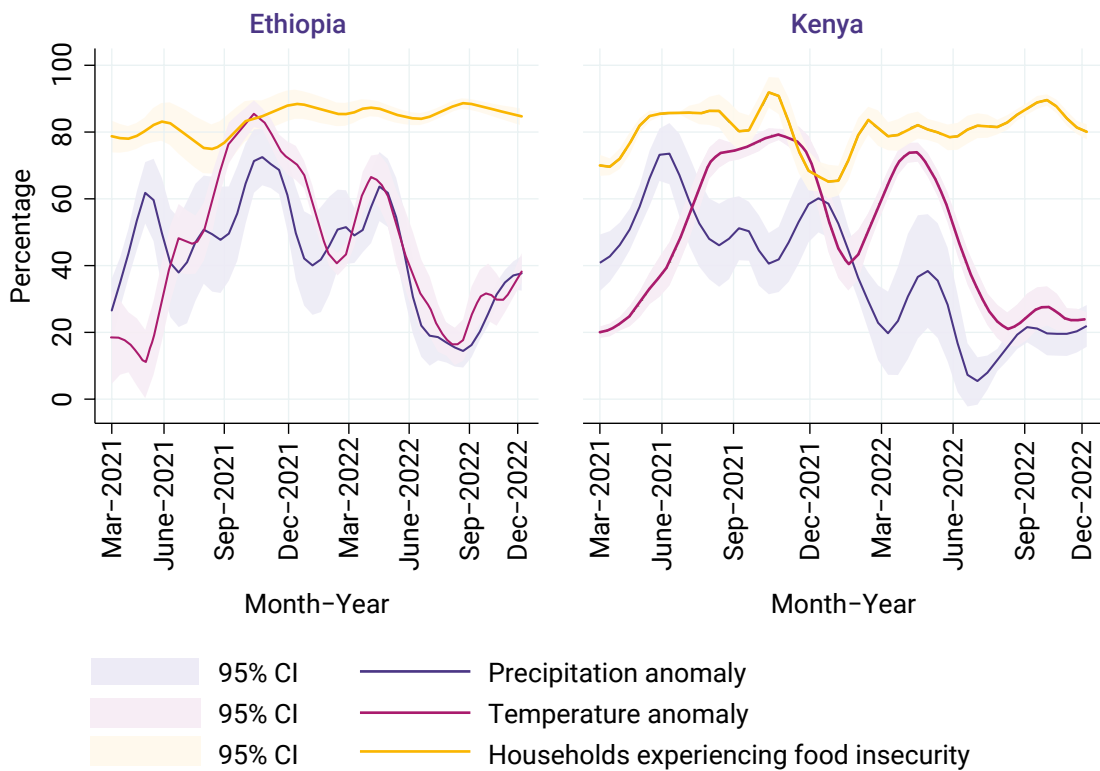
FIGURE 3: TRENDS IN FOOD INSECURITY, TEMPERATURE, AND PRECIPITATION
