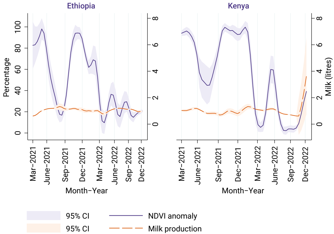
FIGURE 2: TRENDS IN FORAGE CONDITIONS AND MILK PRODUCTION
